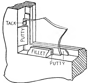
FIG. 444. PLACEMENT OF GLASS PANELS.
